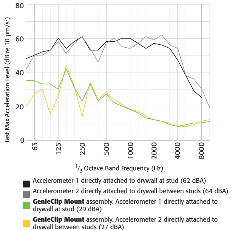
Vibration level on receiver room side of wall due to kitchen cabinet door slams with and without GenieClip Mounts .
